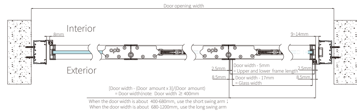
Top view of the door opening
