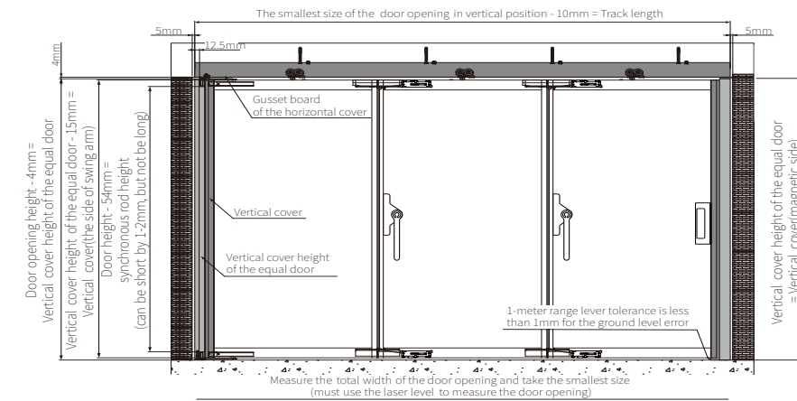
Front view of the door opening
