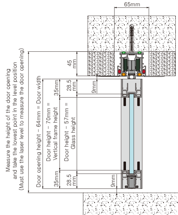
Cross-section of the door opening
